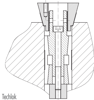
Techlok
