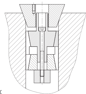
Grayloc
